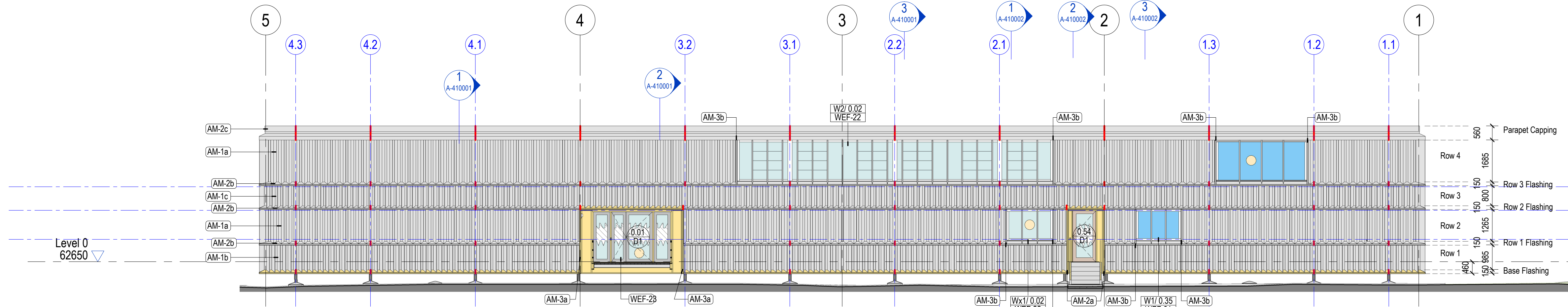
1 East Facade Elavation 1: 100
